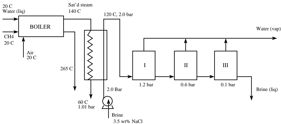
Figure 2: Reference design for multi-stage flash desalination.
